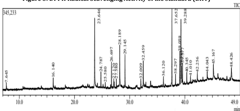
Figure 4: GCMS Profiling
